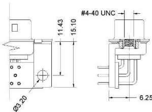
CODE - 4 4-40 UNC INSERT+PCB + THRU HOLE
