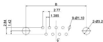
Recommended PCB Layout (Plug and Receptacle)
