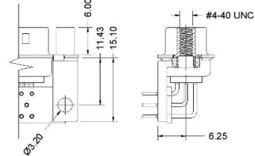
CODE - 6 4-40 UNC STANDOFF+PCB + THRU HOLE
