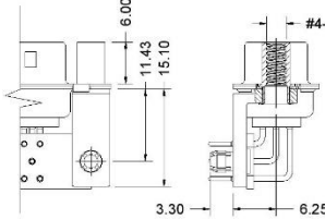
CODE - 5 4-40 UNC STANDOFF+PCB + BOARDLOCK
