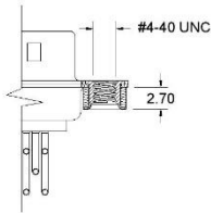
CODE - 5 4-40 UNC STANDOFF+PCB + BOARDLOCK
