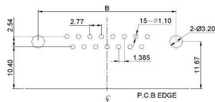
RECOMMENDED P.C.B LAYOUT (FOR PLUG AND RECEPTACLE)
