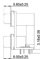
CTR TO CTR VERTICAL SPACING E±0.25 F±0.38 Inch (mm) Inch (mm) .625 (15.88) 1.119 (28.43) .750 (19.05) 1.244 (31.60) .900 (22.86) 1.394 (35.41)
